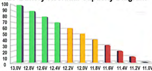
12V Battery Residual Capacity Diagram
